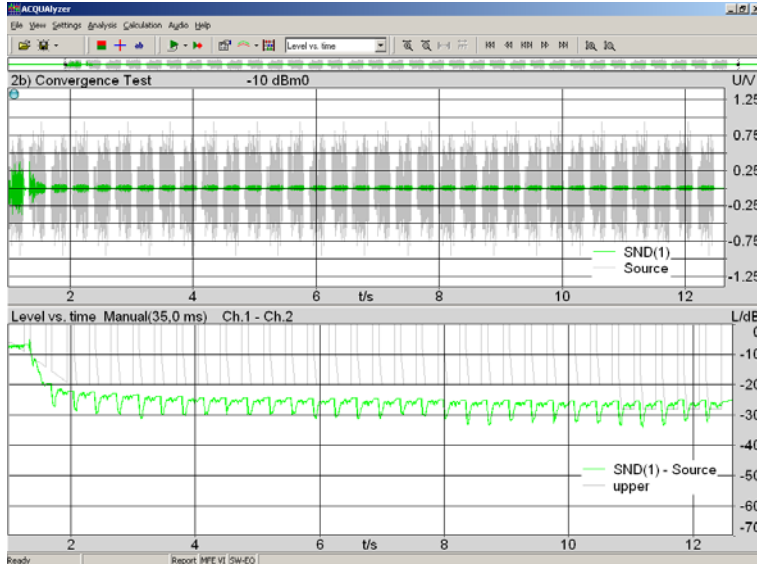
Example of convergence test result in ACQUA analysis module ACQUAlyzer. Upper window: Time sequence (green: measured signal, gray: source signal). Lower window: Level vs. time analysis of measured signal referred to source signal (green) and tolerance scheme (gray).
