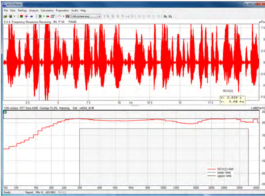
Example: Measurement signal and analysis result of a frequency response measurement
