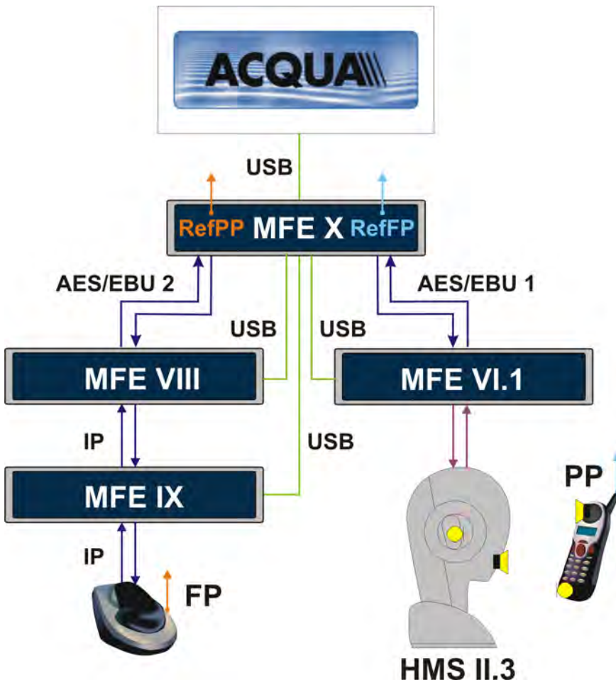
Example configuration: CAT-iq™ acoustic measurements with analysis system ACQUA, artificial head HMS II.3, front ends MFE VI.1, MFE VIII, MFE IX and MFE X.
