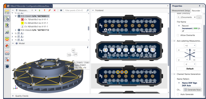
Measurement Setup
