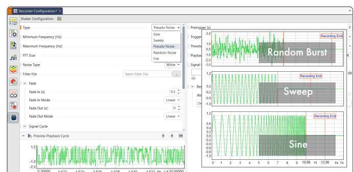
Shaker Configuration
