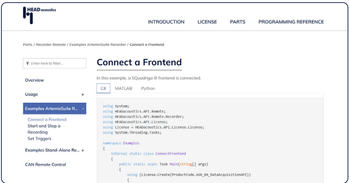
C# programming example: Data Acquisition API (ASX 04)
