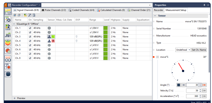
move°S configuration for HSU III.2 head rotation
